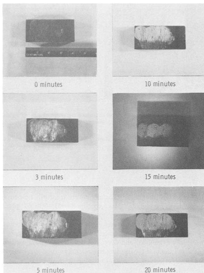
FIG. 5—Copper specimen subjected to cavitation showing serial number restoration at various exposure times (original magnification \times 1 ).
