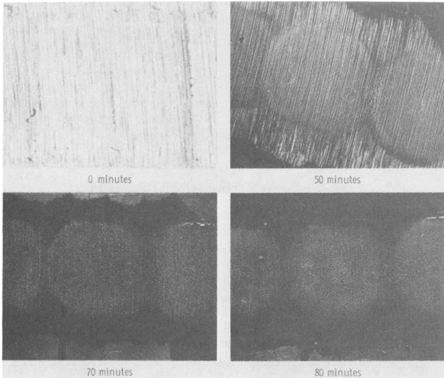
FIG. 10—Brass specimen subjected to cavitation showing serial number restoration at various exposure times (original magnification \times 5 ).
