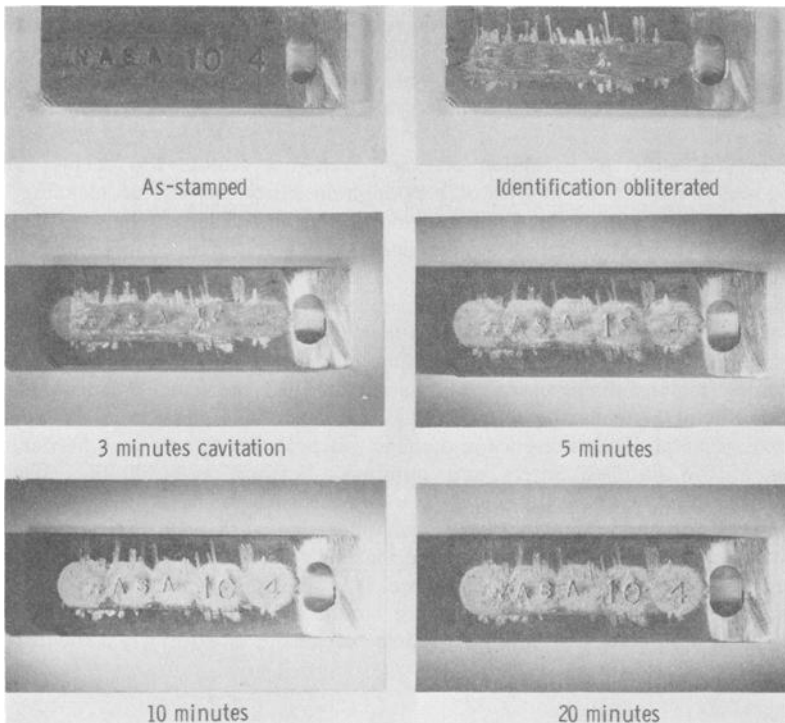
FIG. 18—Results of serial number restoration by cavitation on aluminum specimen (identification stamped and obliterated by NASA).
