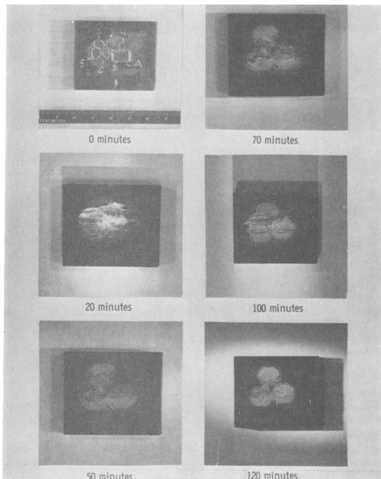
FIG. 11—Steel specimen subjected to cavitation showing serial number restoration at various exposure times (original magnification \times 1 ).
