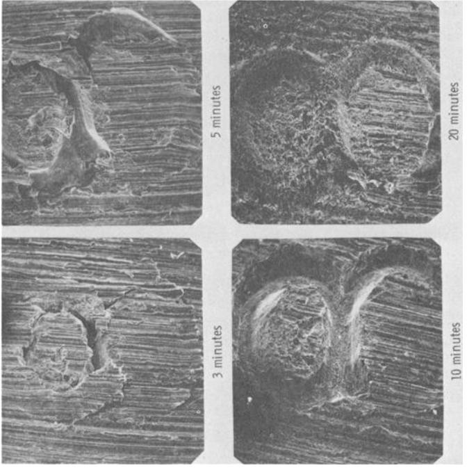
FIG. 8—Scanning electron photomicrographs of the number 8 on the copper specimen in the process of being restored. Smearred metal is being removed from the grooves (original magnification X30).
