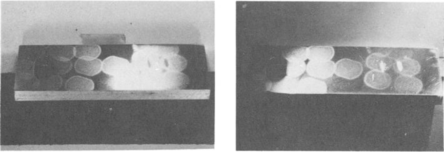
FIG. 4—Polished specimen showing cavitation damage haze patterns caused by exposures from 1 to 30 s at varying separation distances (same specimen at different light angles).
