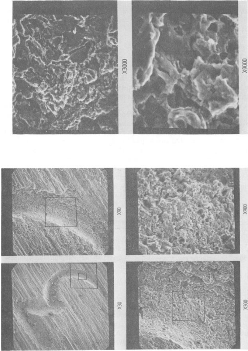
FIG. 16—Scanning electron microscope photomicrographs of restored number 3 on steel at various magnifications after 120-min exposure to cavitation.
