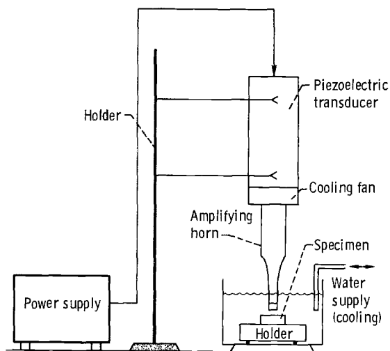
FIG. 3—Schematic diagram of test apparatus used to restore serial numbers by ultrasonically induced cavitation.
