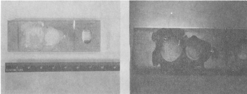
FIG. 17—Aluminum specimen showing results of initial attempt to restore letters and numbers: (a) 1-min cavitation, uniform light and (b) 5-min cavitation, oblique light.
